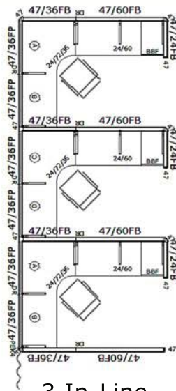
3 In-Line
