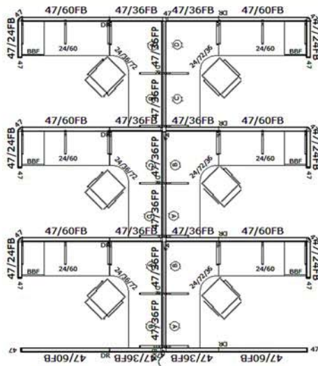
6 Pack
