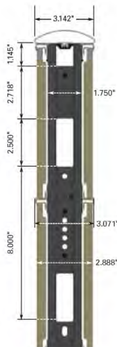
PANEL PROFILE
